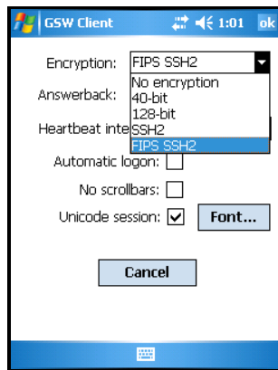
GSW Mobile Client FIPS 140-2 Configuration
