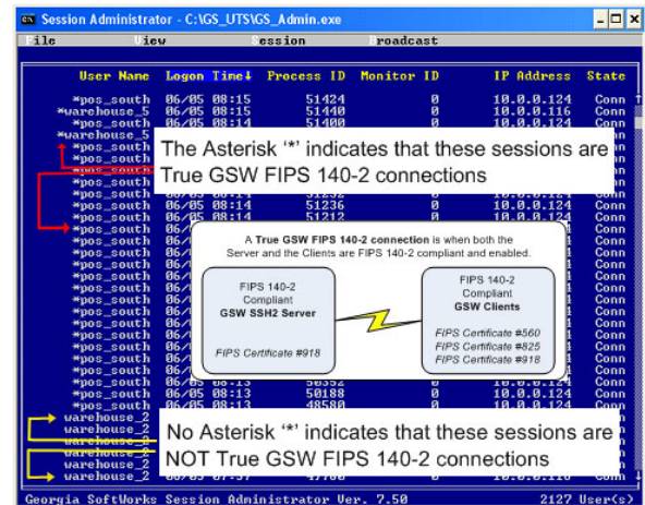
GSW SSH2 Server Session Administrator
